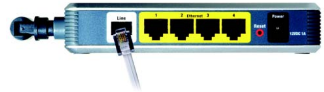
Figure 4-4: Connect the ADSL Line
